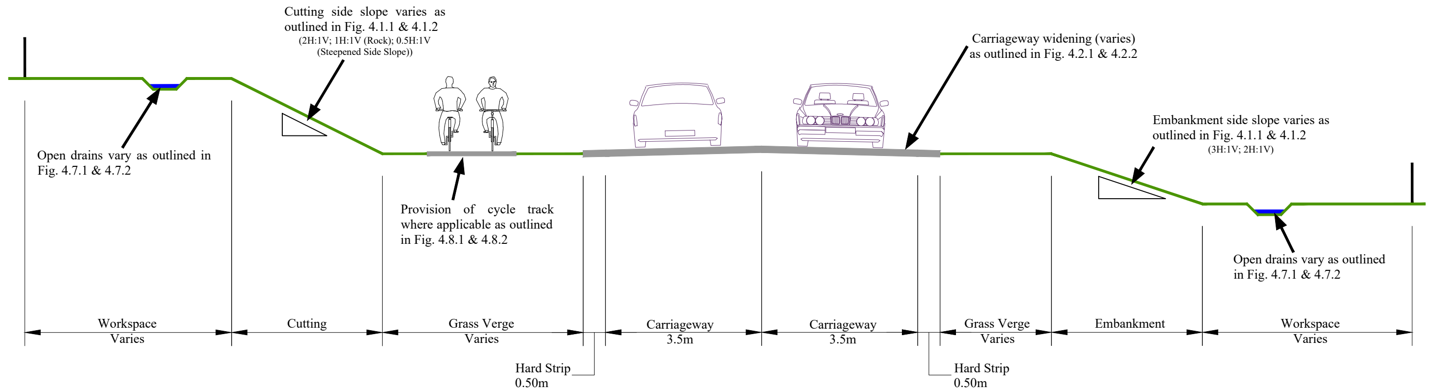
TYPE 2 SINGLE CARRIAGEWAY TYPICAL CROSS SECTION
